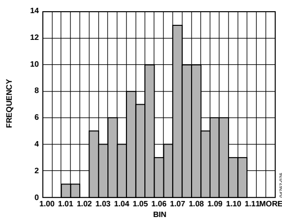
Figure 39. I_{DD} Histogram V_{DD} = 5.0V
